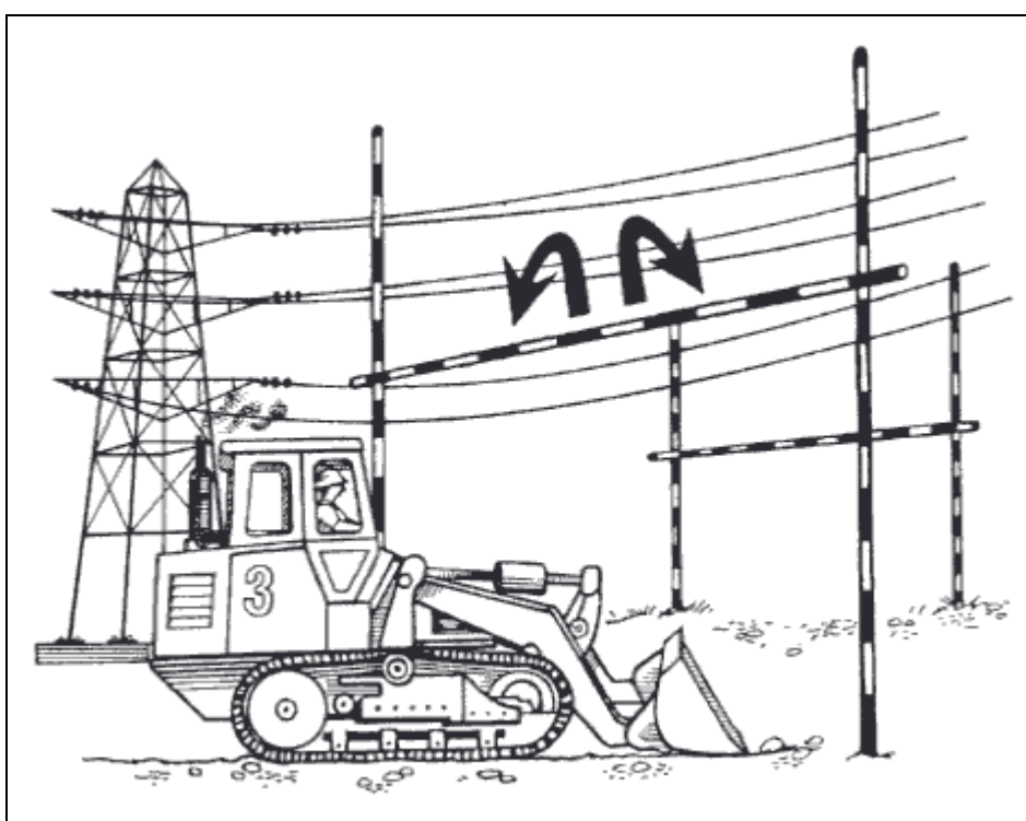
Figure 32. Goalposts to compel drivers to lower crane and excavator jibs, and avoid contact with overhead power lines
