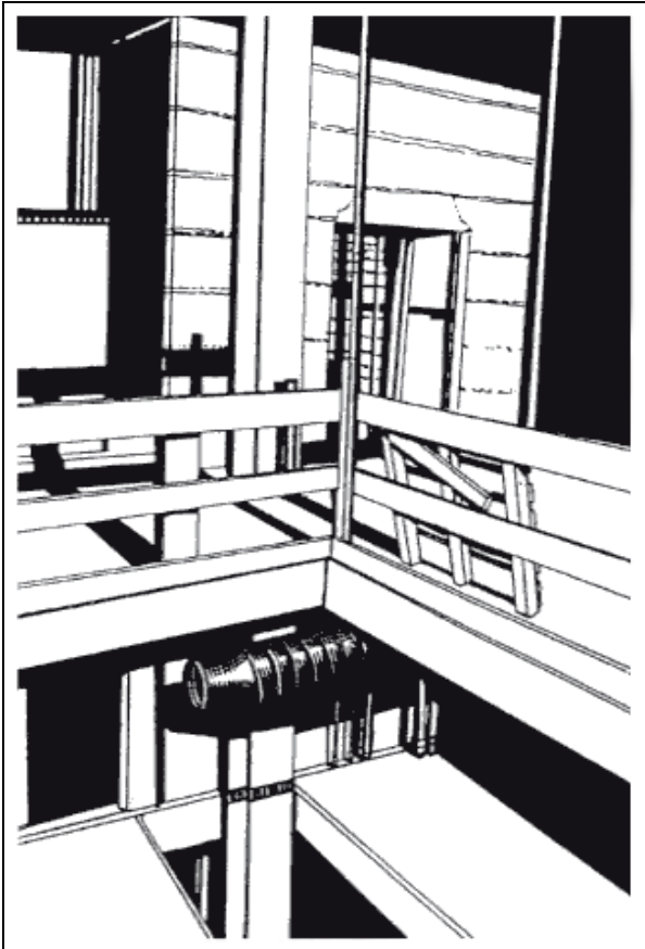
Figure 5. Edge protection: Guard-rails and toe boards at open edges of floors and working platforms to prevent workers from falling
